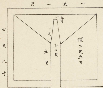
(面平) 竈
